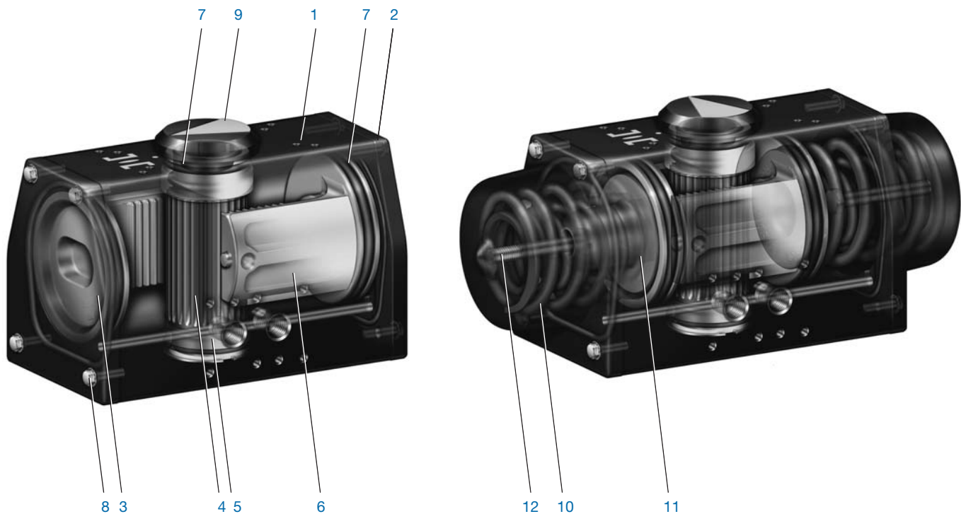
Note: F79U 006 Double Acting actuator illustrated.
